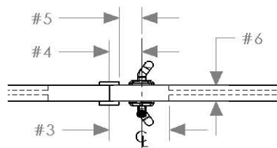
SLIDING DOOR PLAN VIEW
